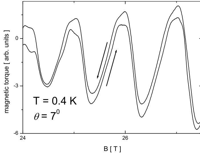
Figure 5.25: The magnetic torque exhibits a strong diamagnetic hysteresis on sweeping the magnetic field up and down, (only) within the CDW_x state.
