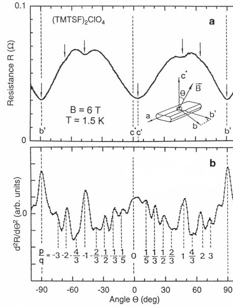
Figure 2.12: a) Q1D AMRO in the organic compound (\text{TMTSF})_2\text{ClO}_4 exhibiting pronounced dips at angles expected from the theory [46]. b) Second derivative of the curve in a) clearly showing the modulated structure. For the definition of p and q see text, from [9].
