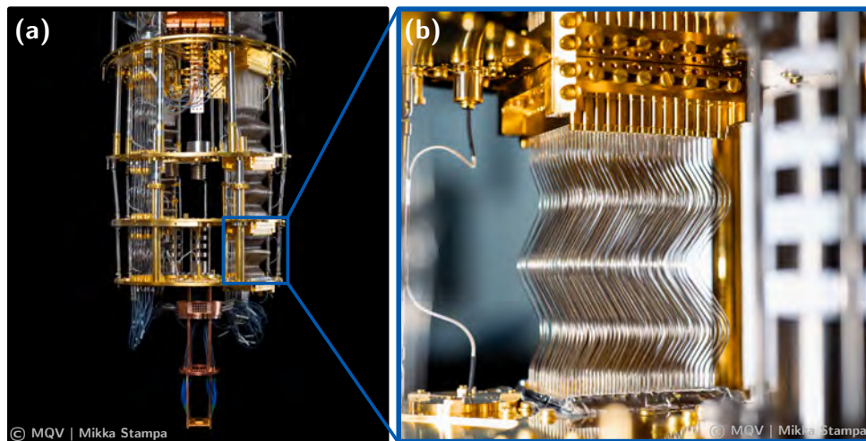
Figure 1: Bluefors XLD1000 system equipped with 400 coaxial lines to support a 100-qubit quantum processor. (a) The complete cryostat without thermal shields is shown, with a quantum chip mounted on a PCB at the bottom and the high-density wiring positioned on the left and right sides of the cryostat. (b) A close-up view of the newly installed high-density wiring highlights the carefully designed bends, which accommodate thermal contractions at cryogenic temperatures.
