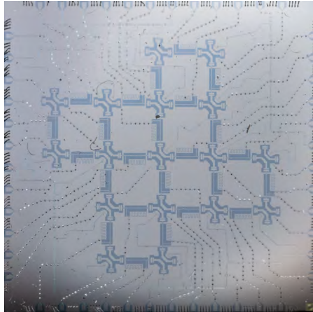
Figure 1: A 17-transmon-qubit demonstrator (with 24 tunable couplers) fabricated by WMI.
