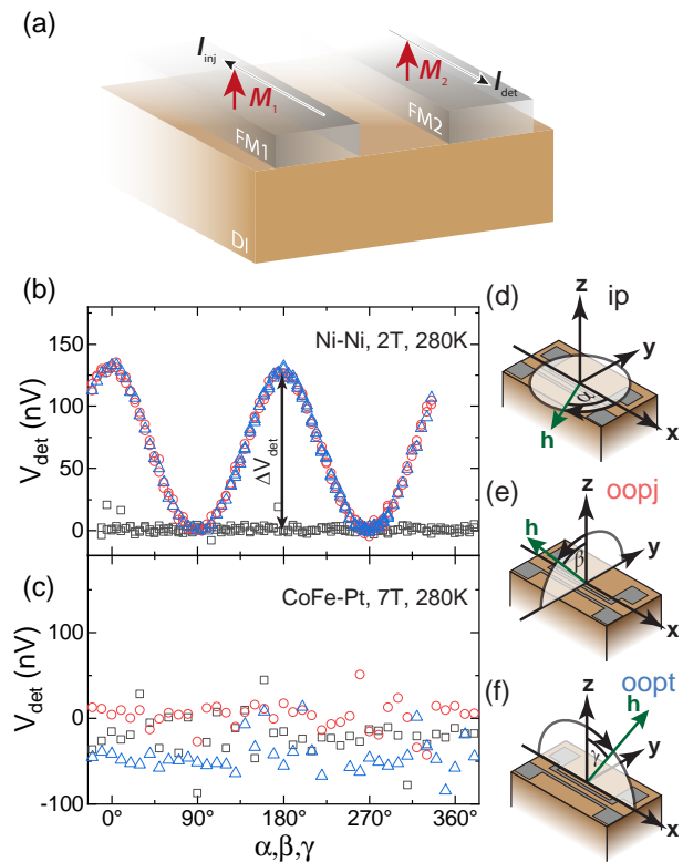
Figure 1: (a) Sketch of the sample geometry with the magnetization M of the ferromagnetic electrodes oriented along the surface normal. (b,c) Angle-dependence of V_{det} for Ni-Ni strips (panel b) and CoFe-Pt strips (panel c) obtained at 280 K and \mu_0 H = 2 T, 7 T. Black squares correspond to ip-rotations, red circles to oopj-rotations and blue triangles to oopt rotations, respectively. (d,e,f) Illustration of the rotation planes used for the angle-dependent measurements: in-plane rotation (d, ip), out-of-plane perpendicular to j (e, oopj), and out-of-plane perpendicular to t (f, oopt).
