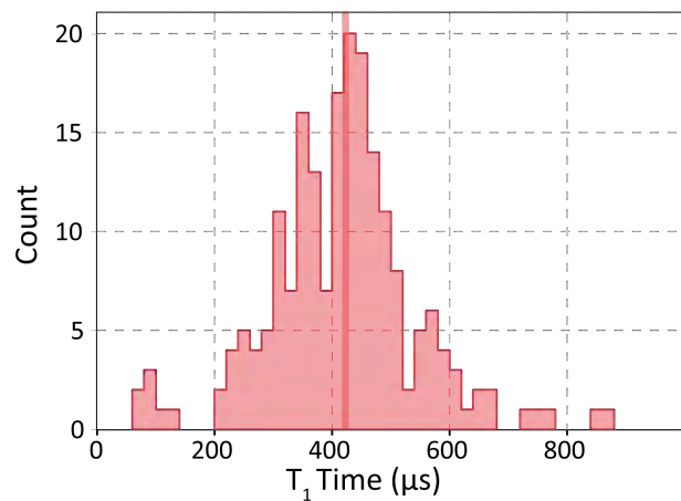
Figure 2: Distribution of transmon qubit T_1 times monitored over 12 hours.
