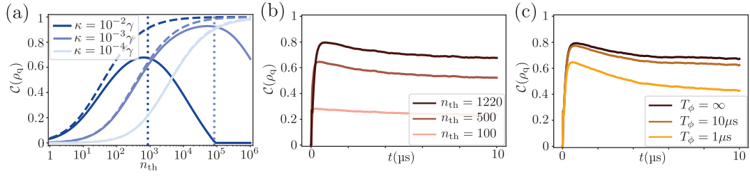
Figure 2: (a) Plot of the steady-state entanglement (expressed in terms of the concurrence \mathcal{C} ) between the two qubits as a function of the number of thermal photons of the source and for different cavity bandwidths \kappa/\gamma . Time evolution of the entanglement under realistic experimental parameters (see main text) for (b) different thermal occupation numbers and (c) at room temperature for different dephasing times T_\phi .
