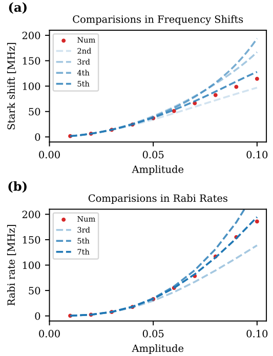
Figure 2: Stark shift (a) and Rabi rate (b) computed at different orders in perturbation theory (dashed lines) compared to the numerical simulation of the dynamics (red dots).
