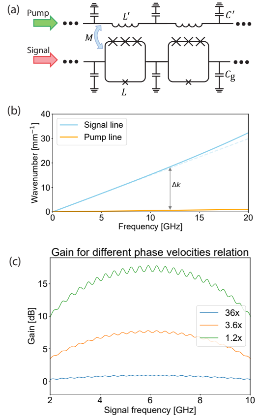
Figure 1: (a) Circuit schematic of a flux-pumped JTWPA based on SNAILs. A linear pump waveguide is inductively coupled to a nonlinear signal medium consisting of SNAILs. (b) Dispersion relation for the signal and the pump lines. (c) Predicted gain of the flux-pumped JTWPA as a function of frequency for varying phase velocity ratios between the pump and signal tones.
