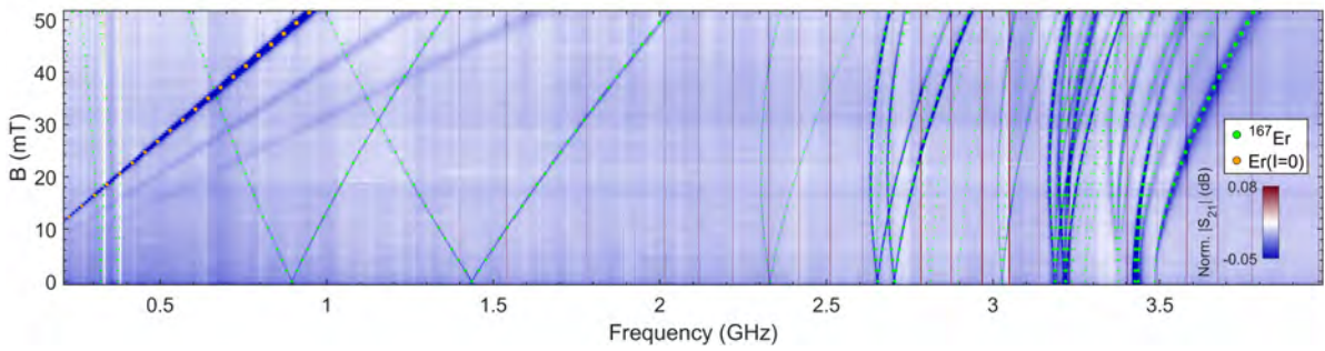
Figure 1: Broadband electron spin resonance allows to probe multiple allowed hyperfine levels of \text{Er} : \text{CaWO}_4 by measuring the microwave absorption as a function of both frequency and magnetic field B . The simulation (green circles) coincides with the experimental data only by assuming a non-vanishing quadrupole tensor \mathbf{Q} .
