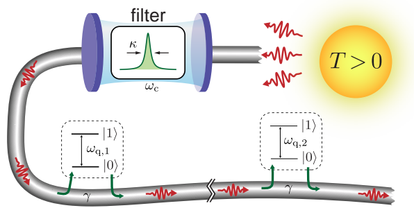
Figure 1: Sketch of the setup considered for entangling two qubits with a non-Markovian thermal source. Here, the source emits incoherent radiation at a high temperature T , which is successively filtered and drives two or multiple qubits along the waveguide. Under resonance conditions, \omega_{q,1} = \omega_{q,2} \simeq \omega_c , and when the bandwidth \kappa of the source is sufficiently small, the qubits relax into a stationary state with a finite amount of entanglement. The amount of entanglement can be systematically increased by raising the temperature T of the source, while reducing its bandwidth.
