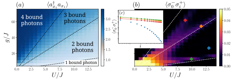
Figure 2: Ground state phases of the bosonic impurity model with 4 excitations per unit-cell. (a) Average photon number of a cavity coupled to a qubit. The number of bound photons depends on the photon-photon interaction U and cavity-atom coupling g . (b) Long-range correlations between the atoms appearing near the transition lines between the different multi-photon bound phases. (c) In green, orange, red, algebraic decay of the atom-atom correlations on the transition lines. In blue, exponential decay of the correlations in the insulating phases.
