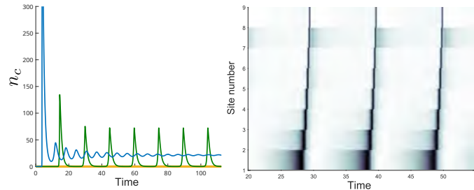
Figure 2: Left: cavity population versus time, showing lasing (blue) and pulsing (green) regimes. Right: space-time plot of the chain population, showing “avalanches” events.
