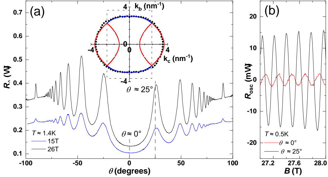
Figure 2: (a) AMRO in \kappa -CN at pressure 0.24 GPa. Inset: the 2D FS determined from the AMRO (black dots) and calculated from the SdH frequencies within the effective dimer model (red and blue). Dashed lines represent the Brillouin zone boundaries. (b) Example of the SdH oscillations at different orientations and pressure 0.24 GPa.
