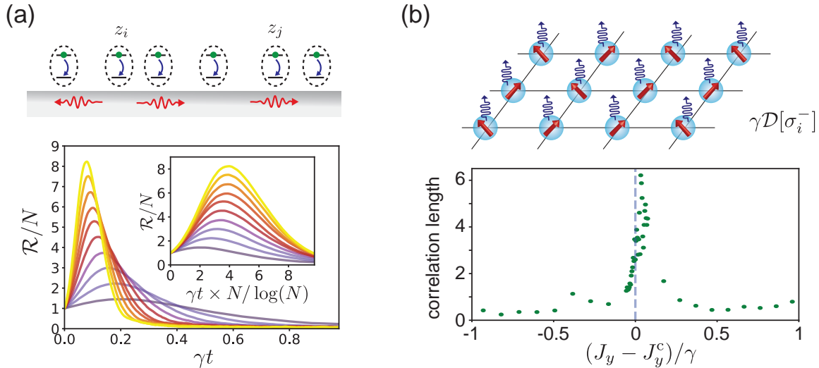
Figure 1: (a) Disordered superradiance. A large number of N two-level emitters with random positions are coupled to a common 1D waveguide. The lower panel shows the time evolution of the average decay rate per qubit, \mathcal{R}/N , with increasing N . (b) Schematic of a 2D dissipative Heisenberg XYZ model. At the critical point J_y^c our DTWA simulations of a spin lattice of size 36 \times 36 clearly capture the expected divergence of the correlation length.
