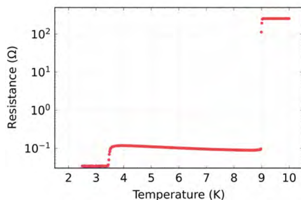
Figure 2: Resistance of a daisy-chains with 18 indium interconnects as a function of temperature.
