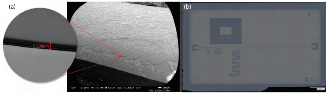
Figure 2: (a) SEM picture of a chip with 2 μm thick layer SrTiO 3 patterned over a superconducting meandered line. (b) Optical photo of a chip with 15 nm thin film of NbTiN with patterned test resonators.
