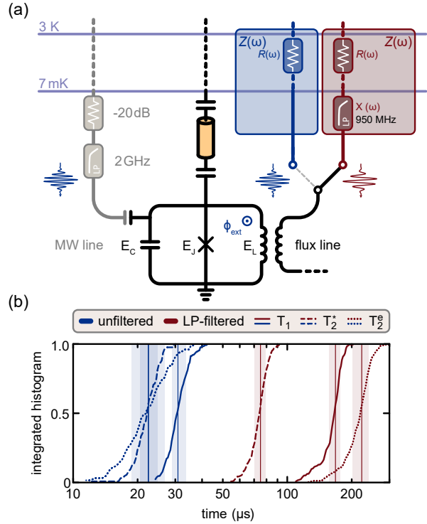
Figure 1: Setup and relaxation times. (a) Setup at the low temperature stages of the cryostat, including readout resonator and two switchable flux line configurations (unfiltered and low-pass (LP) filtered). An additional microwave (MW) line is added for comparison and benchmarking. (b) Integrated histograms for T_1 (solid), T_2^* (dashed), and T_2^e (dotted) for unfiltered (blue) and filtered (red) flux line configuration. Vertical lines with shaded areas illustrate the median and standard deviation.
