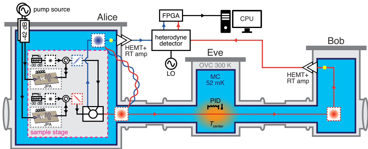
Figure 1: Schematic of our experimental setup for entanglement distribution. Propagating TMS states are generated in Alice. Then, one TMS mode is kept in Alice and another mode is transmitted over the cryolink to Bob. A PID-controlled heater is used to adjust the local temperature T_{\text{center}} in the MC tube at Eve.
