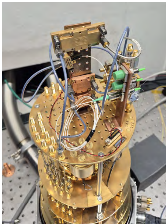
Figure 1: View of an open cryostat with the optical fibers installed. Two samples are mounted and connected to the coaxial and DC lines.
