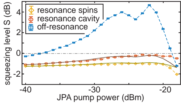
Figure 2: Squeezing level as a function of the JPA pump power for the three different experimental scenarios, as described in the main text. The solid lines represent model predictions based on Eq. 2 using the off-resonance squeezing levels as an input.
