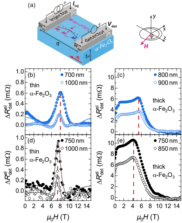
Figure 2: (a) Sample configuration: Pt strips placed on a \alpha -Fe 2 O 3 film in the magnetic (0001) easy-plane phase. The canted sublattice magnetizations M_{1,2} induce a net magnetization M_{net} oriented by an in-plane magnetic field H at angle \varphi , with the Néel order parameter n \perp H . A charge current through the left Pt-electrode generates magnons, detected as a voltage at the right Pt-electrode. (b)-(e) Electrically induced magnon spin signal amplitude \Delta R_{det}^{el}(\mu_0 H) at 200 K for thin (left) and thick (right) films with varying injector-detector separations d (full/open circles). The 19 nm and 89 nm thick AOS-Fe 2 O 3 films (d, e) show higher \Delta R_{det}^{el} than the 15 nm and 103 nm thick NAOS-Fe 2 O 3 films (b), (c). Red dashed lines indicate the compensation fields \mu_0 H_c .
