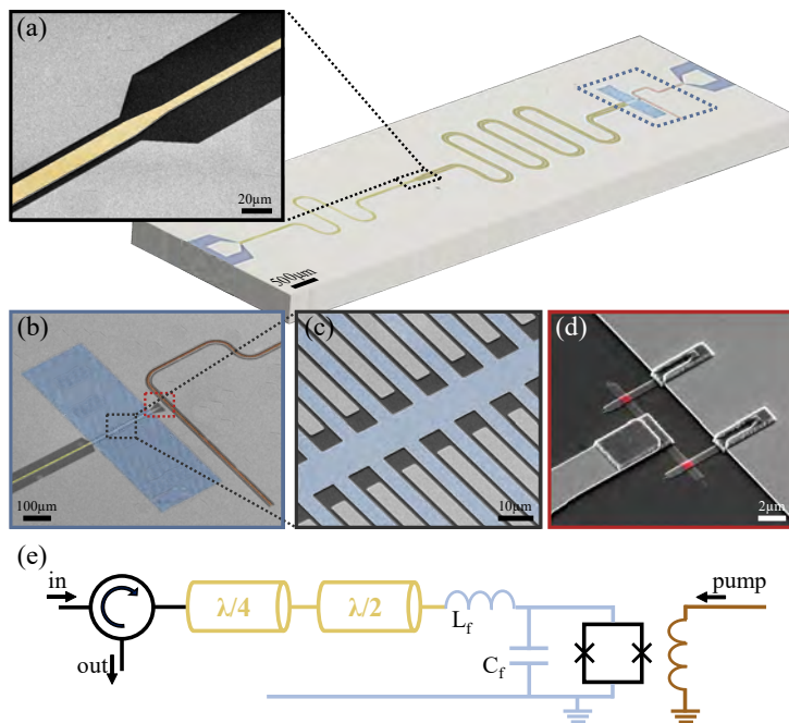
Figure 1: Design layout of the broadband JPA. Colored boxes show close-ups of central elements of the broadband JPA: (a) SEM image of the connection between the \lambda/4 and \lambda/2 CPW resonators. (b) The dc-SQUID area with shunting fish-bone capacitors and a pump line. (c) Detailed view of the fish-bone array geometry. (d) SEM image of the dc-SQUID, with the Al strips forming the Al/AlO x /Al Josephson junctions shown in red. (e) The corresponding circuit diagram.
