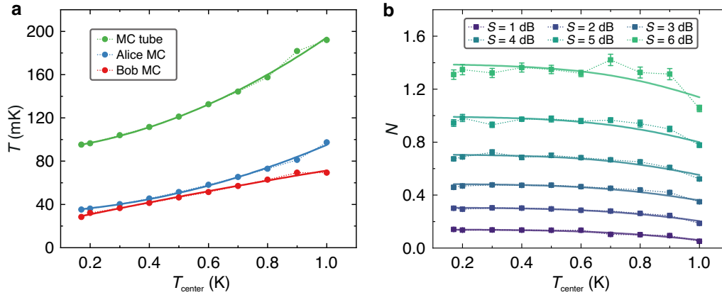
Figure 2: Experimental results. (a) Effect of the cryolink center heating on temperatures of various QLAN components. (b) Negativity, N , of the two-mode, Alice and Bob, state as a function of T_{\text{center}} . Positive negativity, N > 0 indicates bipartite quantum entanglement (inseparability) of microwave modes.
