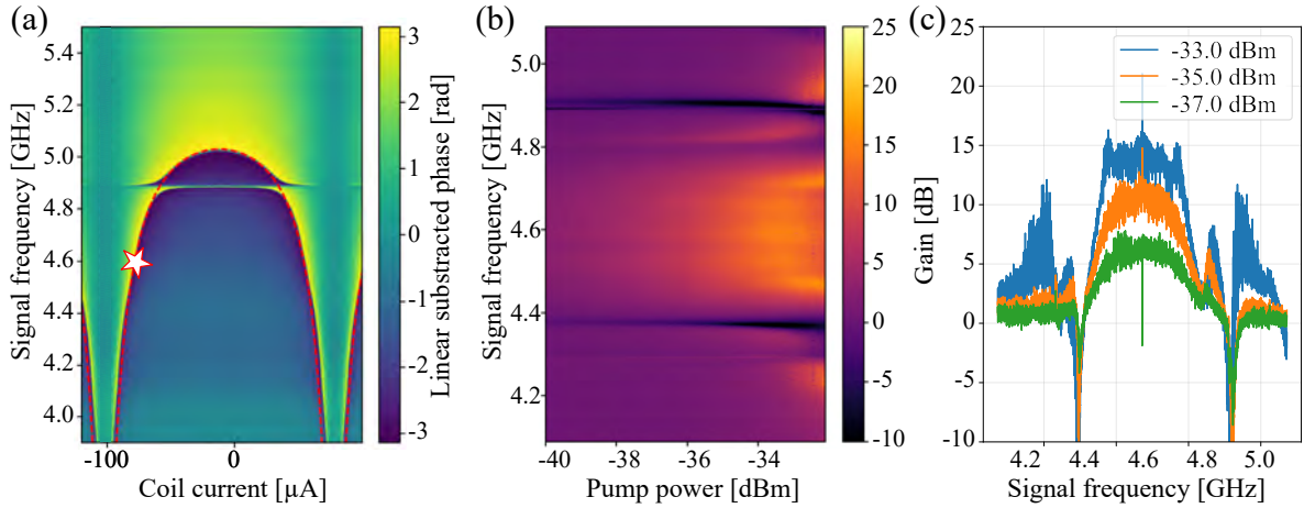
Figure 2: Experimental characterization of the broadband JPA. (a) Flux tuning curve of the broadband JPA. The star symbol indicates the chosen flux working point used in (b). (b) Amplification gain as a function of the pump power and signal frequency, with the pump frequency of 9.18 GHz. Here, the pump powers are referred to the sample pump port. (c) Selected cross-sections of the gain profile.
