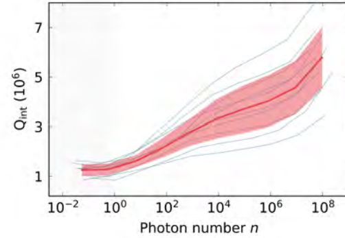
Figure 3: Internal quality factor of 3D integrated resonator as a function of the photon number.
