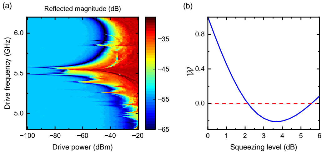
Figure 2: (a) Two-tone spectroscopy measurement as a function of the drive power of the coupled qubit-cavity system. Two narrow resonant responses at the frequencies of f_1 = 5.48 GHz and f_2 = 5.57 GHz represent a quantum polariton state, which can be used for entangling it with the TMS state. (b) Numerical simulation of the entanglement witness \mathcal{W} between the qubit and the propagating TMS state as a function of the squeezing level for typical experimental parameters.
