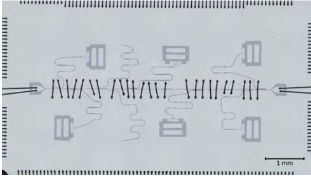
Figure 1: Micrograph of a test chip with six qubits coupled to a common transmission line via CPW resonators. Two additional CPW resonators are available to disentangle losses from the groundplane and the Josephson junctions.
