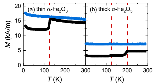
Figure 1: Temperature dependence of magnetization M of \alpha -Fe 2 O 3 films with (a) 25 nm (NAOS-Fe 2 O 3 , blue) and 19 nm (AOS-Fe 2 O 3 , black) and (b) 103 nm (blue) and 89 nm thickness (black). Red dashed lines indicate the Morin transitions in AOS-Fe 2 O 3 . Measurements were conducted while heating the samples in an in-plane magnetic field of \mu_0 H = 100 mT after zero-field cooling. A diamagnetic background signal was subtracted from the data.
