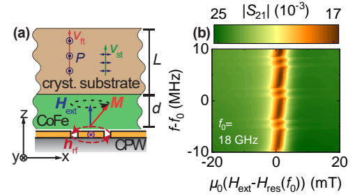
Figure 1: (a) Schematic of the bulk acoustic wave resonator mounted on top of a CPW. The driven ferromagnetic resonance mode can couple to the transverse acoustic phonon modes that form standing waves in the sample. (b) Microwave transmission magnitude S_{21} as a function of the external magnetic field \mu_0 H_{\text{ext}} around H_{\text{res}}(f_0) = 3.005 T and the applied microwave frequency f around f_0 = 18 GHz measured at T = 5 K.
