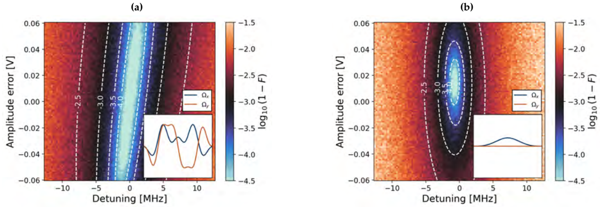
Figure 1: Gate infidelity 1 - F (Eq. 3) for (a) robust gates derived from a Fourier series parametrization and (b) Gaussian pulses with DRAG corrections, with various amplitude and detuning errors, simulated using Eq. 1. To highlight the differences, the gate infidelity is shown on a log scale. The contour lines correspond to gate fidelities of 99.99% to 99.68%. Corresponding pulse envelopes for the gates with a length of 100 ns are shown in the insets.
