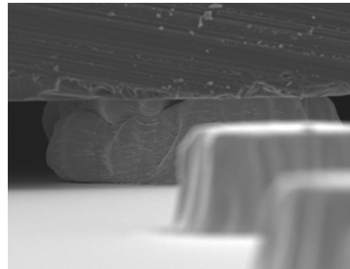
Figure 1: SEM picture of an indium-based interconnect, consisting of two separate indium bumps that were thermally compressed.
