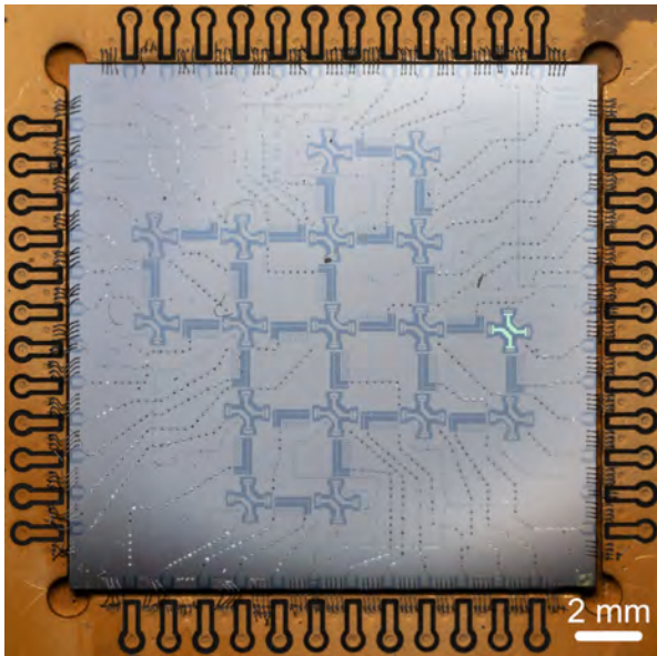
Figure 1: Optical image of a 17-qubit chip with qubits at the corners of rectangular plaquettes connected by tunable couplers. Qubit 11 is highlighted in green.
