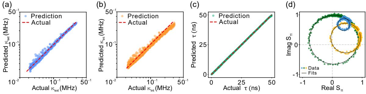
Figure 2: Performance of KAPPANET on test data in predicting parameters (a) \kappa_{\text{ext}} , (b) \kappa_{\text{int}} , and (c) \tau . (d) Predictions of KAPPANET fit well to the actual test data over a large range of coupling rates including the overcoupled \kappa_{\text{ext}} > \kappa_{\text{int}} (green), critically coupled \kappa_{\text{ext}} \sim \kappa_{\text{int}} (gold), and undercoupled \kappa_{\text{ext}} < \kappa_{\text{int}} (blue) resonator regimes.
