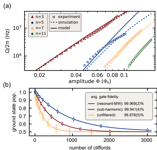
Figure 2: Rabi frequencies for n -photon sub-harmonic drives. (a) Rabi frequencies \Omega_n as a function of pulse amplitude \Phi for different sub-harmonic drives, compared to numerical simulation and an analytic model. (b) Randomized benchmarking for different single-qubit gate implementations. The fidelity is determined from the ground state population as a function of number of random Clifford gates averaged over 24 hours.
