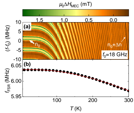
Figure 2: (a) Difference of the fitted FMR linewidth \Delta H and the base linewidth \Delta H_0 as a function of microwave frequency f around f_0 = 18 GHz and temperature T . (b) Free spectral range f_{\text{FSR}} as a function of T . The red continues line shows the calculated theoretical behavior using Eq. (1).
