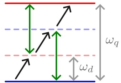
Figure 1: Subharmonic Rabi model. Diagrammatic representation of the lowest order Rabi rate for a three-photon process. The blue and red solid lines represent the initial and final states. The black arrows represent energy increase after the photon absorption and transition to a virtual Floquet state (dashed lines). The green arrows indicate the weight by which each step in the process is suppressed.
