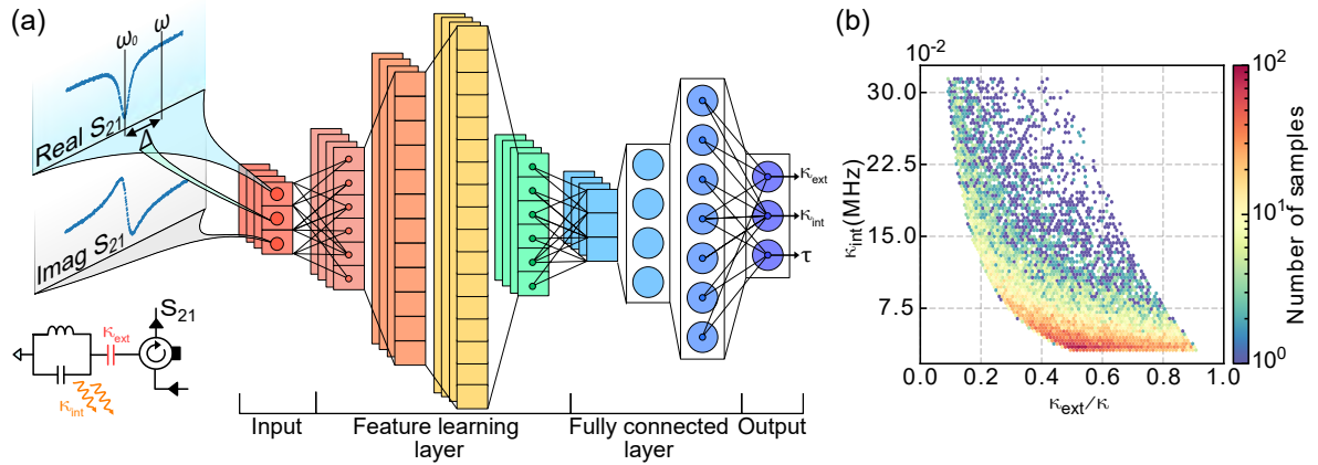
Figure 1: (a) Illustration of KAPPANET, the physics-informed neural network based on six convolutional layers and three fully connected layers. The three inputs to KAPPANET are \text{Re } S_{21} , \text{Im } S_{21} , and detuning \Delta = \omega - \omega_0 . Outputs from KAPPANET are the predicted coupling rates \kappa_{\text{ext}} , \kappa_{\text{int}} , and the cable delay \tau . (b) Distribution of \kappa_{\text{int}} versus coupling efficiency \kappa_{\text{ext}}/\kappa used for generation of synthetic scattering coefficients in the training dataset. The dataset consists of 20 \times 10^4 noisy resonators with randomly sampled coupling rates \kappa_{\text{ext}} , \kappa_{\text{int}} , and the cable delay \tau .
