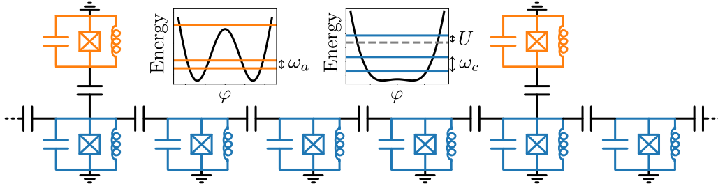
Figure 1: Waveguide QED with interacting photons. The two-level emitters (in orange) are realized by highly non-linear superconducting circuits. The waveguide is a chain of capacitively coupled superconducting circuits. Their anharmonicity U induces interaction between the photons propagating in the waveguide.
