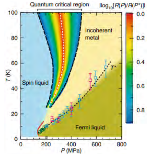
Figure 1: Phase diagram of \kappa -CN from [1].
