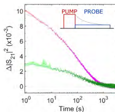
Figure 2: Saturation recovery reveals long lifetimes of the hyperfine states. The relaxation is fitted (blue solid line) to a sum of three exponential functions to account for various decay channels involving intermediate states. (Magenta) 2.65361 GHz transition with lifetimes \tau_1 = 8.2\text{ s} , \tau_2 = 74\text{ s} , \tau_3 = 335\text{ s} . (Green) 3.02655 GHz transition with lifetimes \tau_1 = 7.9\text{ s} , \tau_2 = 125\text{ s} , \tau_3 = 711\text{ s} .
