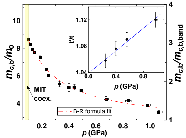
Figure 3: Pressure-dependent cyclotron mass (main panel) and frustration ratio (inset) in \kappa -CN.
