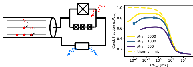
Figure 3: Left: alternative design for non-reciprocal transport, using a superconducting waveguide coupled to a dissipative element. Right: population fraction in the lowest mode versus temperature. Below a certain critical temperature, a macroscopic number of excitation accumulate in the ground mode, an evidence of Bose-Einstein condensation.
