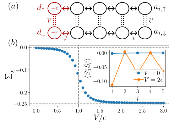
Figure 3: (a) Double chain of bosonic modes encoding the Anderson fermionic impurity model after Jordan-Wigner transformation. The Coulomb interaction translates into a cross-Kerr interaction (double dashed lines). The detuned first site encodes the impurity. (b) Long-range correlations of the Kondo singlet appear when increasing the impurity cross-Kerr interaction V .
