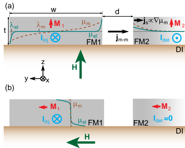
Figure 2: (a) Spin transport experiments with the magnetic field pointing out of the sample plane. Charge-to-spin conversion leads to an electronic spin accumulation \mu_{el} at the edges of the FM1 layer upon application of a current I_{inj} with the spin polarization oriented along the magnetization \mathbf{M} . The electronic spin accumulation gives rise to a magnon chemical potential \mu_m , which relaxes on the scale of the magnon diffusion length \lambda_m , which exceeds the electronic spin diffusion length \lambda_{el} . The finite magnon accumulation at the right side couples to the thermal magnon bath in the FM2 strip by dipolar coupling and via phonon spin transport through the DI and thereby induces a dc current I_{det} in the FM2 strip by spin-to-charge conversion. (b) Illustration of the chemical potential profiles for \mathbf{M} within the sample plane. The electron spin accumulation is now at the top and bottom surfaces and fails to generate any substantial magnon chemical potential as t \ll \lambda_m . Thus, no angular momentum transport signal is observed in the detector.
