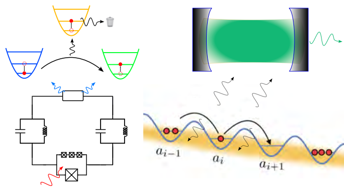
Figure 1: Left: illustration of dissipation-assisted nonreciprocal transfer. Right: generalization to an extended chain. As particles hop along the chain, part of the energy they emit is stored in a cavity mode, the rest dissipates into the environment.
