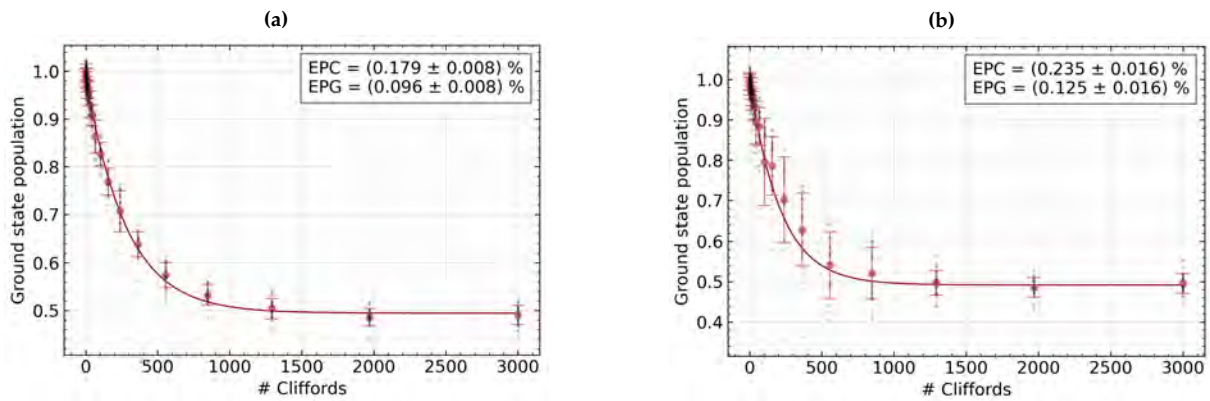
Figure 2: Randomized benchmarking for (a) robust gates derived from a Fourier series parametrization and (b) Gaussian pulses with DRAG corrections. The error per Clifford (EPC) and error per gate (EPG) are estimated by fitting an exponential function to the experimental data.
