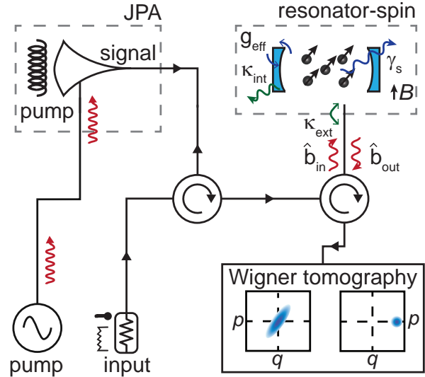
Figure 1: Scheme of the experimental setup. System parameters are from the Hamiltonian in Eq. 1 which provides a detailed model for interactions between the external microwave signals and the resonator-spin system. For each output signal, we perform a Wigner tomography using a Planck spectroscopy which is experimentally realized with an input heatable attenuator. Color plots depict exemplary Wigner functions.
