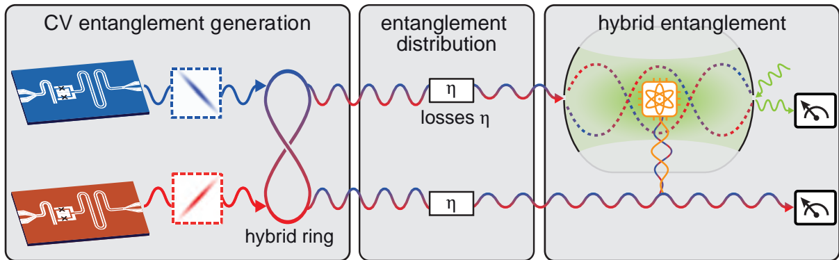
Figure 1: Schematic illustration of the hybrid entanglement protocol. A pair of JPAs is used to generate the propagating TMS states, which act as a quantum-correlated reservoir. A superconducting transmon qubit inside a 3D cavity is then resonantly driven by one of the TMS state modes.
