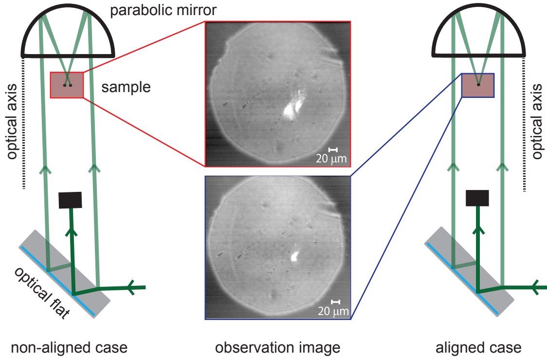
Figure 4.7: Ray diagrams of two different alignment cases. The alignment quality is determined by co-focusing of two laser beams using the optical flat. In the non-aligned case, two spots are visible in the reference image indicating that either the incident beams are not parallel to the optical axis of the parabolic mirror or the sample is not in the focus of the parabolic mirror. In the aligned case, the laser beams and the sample position are adjusted to make the two focal spots to coincide.
