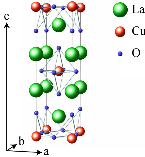
Figure 5.2: Crystal structure ( T -structure) of \text{La}_2\text{CuO}_4 . The conventional unit cell contains two \text{CuO}_2 planes. The copper atom (red) in the center is surrounded by four \text{La}^{3+} atoms (green) on each side. Each of the Cu atoms is surrounded by octahedra of O atoms (blue). Adopted from Ref. [209].
