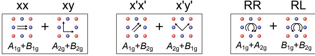
Figure 5.6: Illustration of six different polarization configurations. The black arrows indicate the polarization vectors of the incident and scattered light for each \text{CuO}_2 plane. Each polarization configuration results as the sum of two symmetry components. The red and blue solid circles denote copper and oxygen atoms, respectively.
