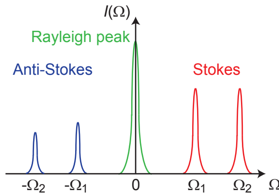
Figure 3.2: A Raman spectrum with different excitations. The Raman intensity I(\Omega) is plotted as a function of the Raman shift ( \Omega ). The peak at \Omega = 0 originates from elastically scattered light. The Stokes ( \Omega > 0 ) lines have higher intensity in comparison to the anti-Stokes ( \Omega < 0 ) lines.
