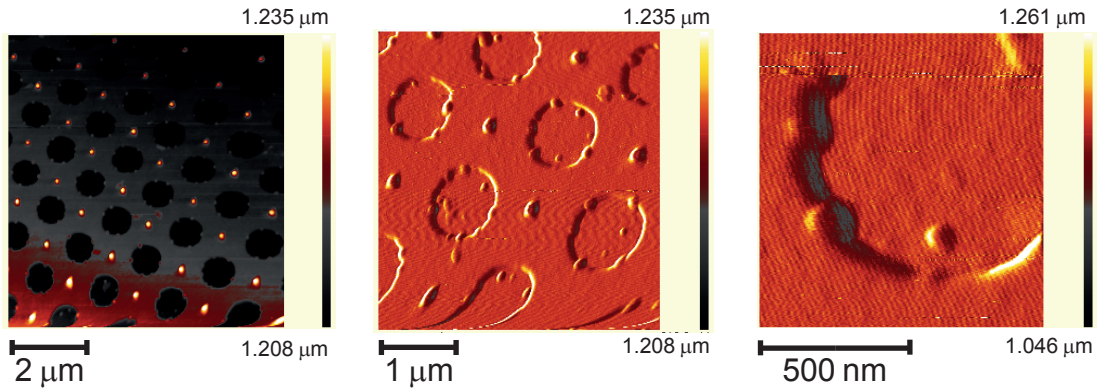
Figure 4.15: Topographic images of a resolution test grid using the tuning fork based AFM in tapping mode. The vertical scale displays the height profile with color code. The scanning patterns were obtained in the backward direction.
