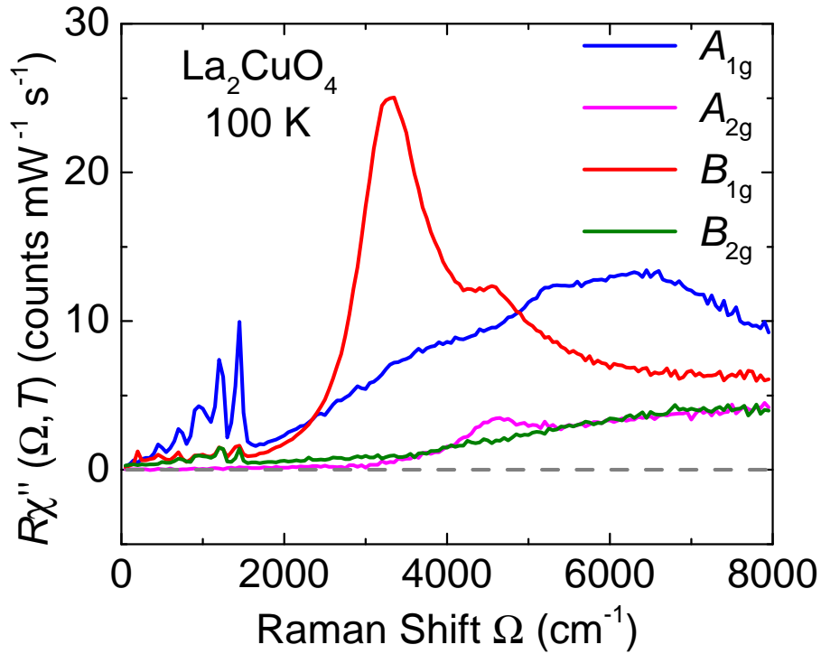
Figure 5.11: Raman spectra of four pure symmetries ( A_{1g} , A_{2g} , B_{1g} , and B_{2g} ) observed in the ab-plane of \text{La}_2\text{CuO}_4 in the AF state at 100 K.
