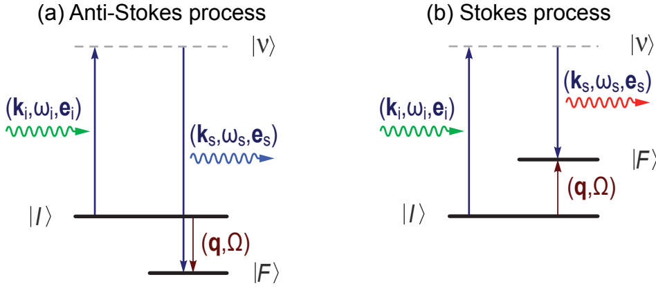
Figure 3.1: Raman scattering processes in the form of energy level diagrams: (a) Anti-Stokes process with an excitation annihilated in the sample resulting in the blue-shifted scattered photons. (b) Stokes process with an excitation created in the sample resulting in the red-shifted scattered photons. The incident and scattered photons are characterized by (\mathbf{k}_i, \omega_i, \mathbf{e}_i) and (\mathbf{k}_s, \omega_s, \mathbf{e}_s) , respectively. Here \mathbf{k} , \omega , and \mathbf{e} define the momentum, energy, and the complex polarization vector, respectively.
