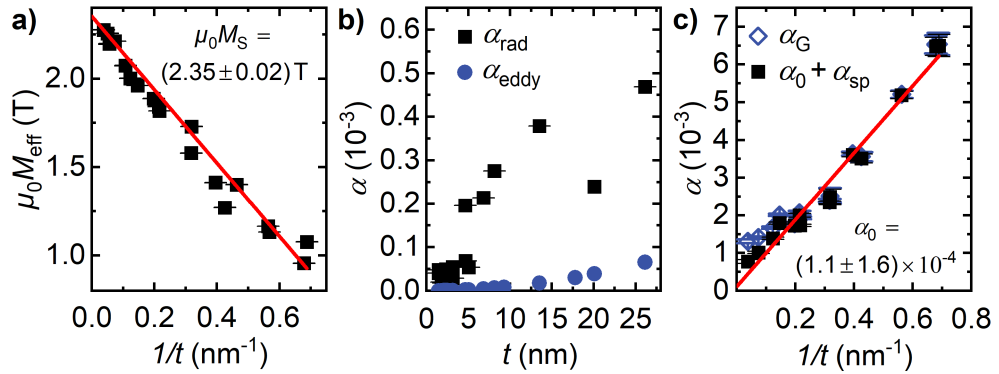
Fig. 3.3. – a) The effective magnetization \mu_0 M_{\text{eff}} scales with reciprocal thickness indicating the presence of an uniaxial interface anisotropy. From the extrapolation to bulk thicknesses t \rightarrow \infty the saturation magnetization M_S can be determined. b) Radiative and Eddy current contributions to the Gilbert damping parameter according to Eq. (3.2) and Eq. (3.4). c) The total Gilbert damping \alpha_G as measured by FMR and the remaining intrinsic and spin pumping contribution after subtraction of the values shown in b).
