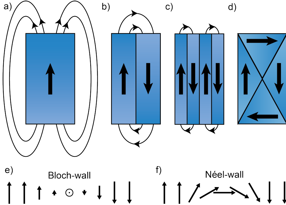
Fig. 4.1. – a) - d) The large stray field induced by a net magnetization and its resulting energy penalty can be reduced by the formation of smaller magnetic domains. However, domain wall energy resulting from the exchange energy has to be paid. In presence of anisotropies the domain size and shape can be redefined. If the anisotropic energy density is very large, domains with unaligned directions can become extinct leading to a remanent configuration as depicted in c) instead of d). The domain walls itself are regions of transition between two distinct domains which depending on its geometry are classified as Bloch-walls (e) and Néel-walls (f).
