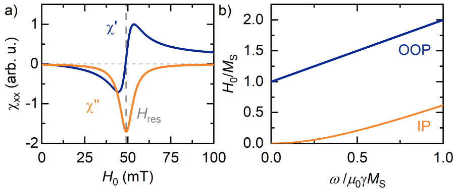
Fig. 2.2. – a) Schematic of the first entry of the Polder susceptibility depending on the external magnetic field strength with the real part \chi' and the imaginary part \chi'' indicating the absorption. Here, a frequency of 10 GHz, \mu_0 M_S = 1.5 T, \mu_0 H_k = 0 , Landé-factor g = 2.1 and \alpha_G = 0.02 was used for a thin film with the external magnetic field applied in-plane (IP). b) Schematic of the Kittel equation of the resonance field for the IP (see Eq. (2.21)) and out-of-plane (OOP, see Eq. (2.23)) geometry.
