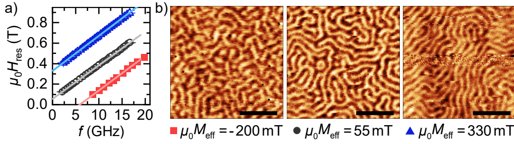
Fig. 5.2. – a) Ferromagnetic resonance of three CoFe multilayers with different FM layer thicknesses of nominally 0.9 nm, 1.1 nm and 1.3 nm. From the fits to Eq. 2.23 we obtain effective magnetizations \mu_0 M_{\text{eff}} = -200 mT, 55 mT and 330 mT, respectively. b) MFM images of the three samples in remanence showing labyrinthine magnetic texture. The domain periodicities determined from Fourier transform correspond to wavelengths of 104 nm, 94 nm and 89 nm, respectively. The black scale bars indicate 500 nm.
