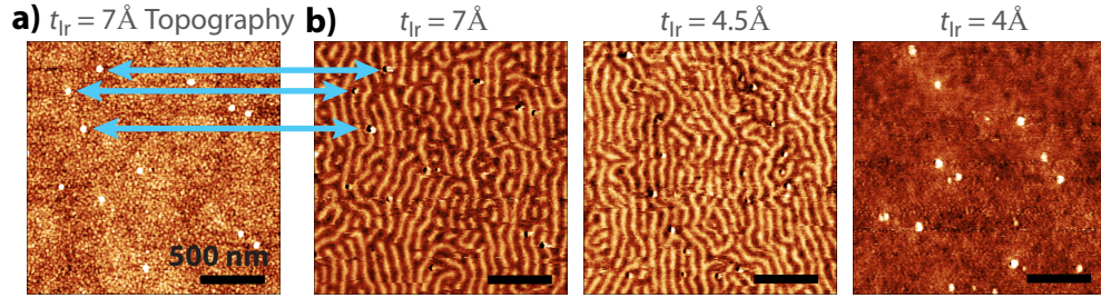
Fig. 5.16. – a) AFM image of the t_{\text{Ir}} = 7 \text{ \AA} investigated in Fig. 5.15 showing the topography with several grains visible as white dots. These dots cause a cross talk in the MFM images shown in b) and thus, circular textures in the MFM images at the corresponding sites do not stem from magnetic stray fields. In b) MFM images of three samples corresponding to ferromagnetic RKKY coupling ( t_{\text{Ir}} = 7 \text{ \AA} ), small antiferromagnetic RKKY coupling ( t_{\text{Ir}} = 4.5 \text{ \AA} ) and stronger antiferromagnetic RKKY coupling ( t_{\text{Ir}} = 4 \text{ \AA} ). For t_{\text{Ir}} = 4.5 \text{ \AA} , a labyrinthine magnetic state is still observed despite the antiferromagnetic coupling. For samples t_{\text{Ir}} \leq 4 \text{ \AA} , where the AFM coupling becomes stronger, no magnetic contrast is observed. The bright dots stem from topographic cross talk.
