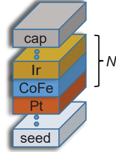
Fig. 5.1. – Simplified sketch of the multilayers investigated where the trilayers are repeated N times.
