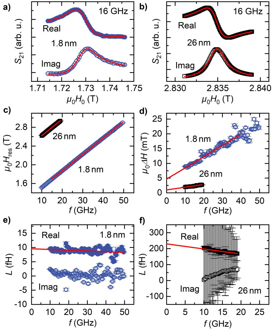
Fig. 3.2. – a),b) Exemplary raw data of the measured microwave transmission S_{21} of blanket Ta(3 nm)/Al(3 nm)/Co 25 Fe 75 ( t )/Al(3 nm)/Ta(3 nm) samples with CoFe thickness t = 1.8 nm (a) blue symbols and t = 26 nm (b) black symbols), respectively. The traces are recorded at 16 GHz with an applied magnetic field H_0 in OOP geometry. The red lines are obtained by fitting Eq. (2.26) to the data. c) and d) show the thus extracted resonance fields H_{\text{res}} and linewidths \Delta H as a function of the applied microwave frequency, respectively. The fit errors shown as error bars are smaller than the symbol size. In c) H_{\text{res}} is fitted to Eq. (2.23) to extract the Landé-factor g and the effective magnetization M_{\text{eff}} . In d) \Delta H is plotted vs. frequency. With a fit to Eq. (2.25) (red lines) the Gilbert parameter \alpha_G and the inhomogeneous linewidth broadening H_{\text{inh}} are extracted. The linewidth of the t = 26 nm thick sample is shown in Fig. 3.4 on an expanded scale. e) and f) depict the complex inductance L of the two samples, where the red lines are linear fits to extract the zero-frequency inductance \tilde{L}_0 . The zero-frequency offset is used to quantify the radiative damping contribution. The large error bars in f) stem from a larger uncertainty of the complex background offset due to the reduced field range of the resonance.
