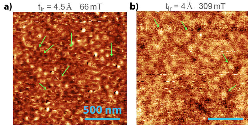
Fig. 5.17. – The antiferromagnetically coupled multilayer with t_{\text{Ir}} = 4.5 \text{ \AA} shows skyrmion formation at finite fields. The green arrows indicate unknown magnetic textures which appear like "popped" bubbles. Even the sample with stronger AFM coupling, which does not show any magnetic contrast in remanence shows circular magnetic textures at finite applied fields some of which are highlighted by green arrows as well.
