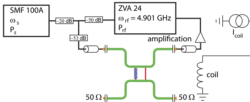
Figure 4.19: Schematic of transmission measurement setup used for two-tone spectroscopy. The frequency \omega_{\text{rf}} is here at a constant value ( \omega_{\text{rf}} = 4.901 \text{ GHz} ) and a second tone with frequency \omega_s and power P_s is applied to the system.
