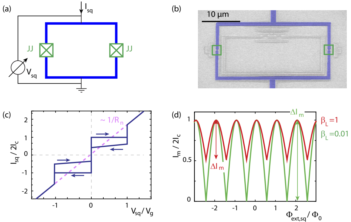
Figure 2.2: dc SQUID: (a) Schematic of a current biased dc-SQUID. The Josephson junctions (green) are symbolized with boxed crosses. By biasing the SQUID with a bias current I_{sq} the voltage V_{sq} is measured. (b) False-colored scanning electron micrograph of a sample. The dc-SQUID is colored blue and the Josephson junctions are highlighted with green boxes. (c) Schematic current-voltage characteristics for a SQUID. For I_{sq} < 2I_c the voltage across the SQUID is zero. At I_{sq} = 2I_c the voltage drops to the a finite value, V_g . With increasing bias current, the current-voltage characteristics follows the normal resistance R_n slope. (d) Two calculated, typical I_m(\Phi_{ext}) characteristics for different values of \beta_L .
