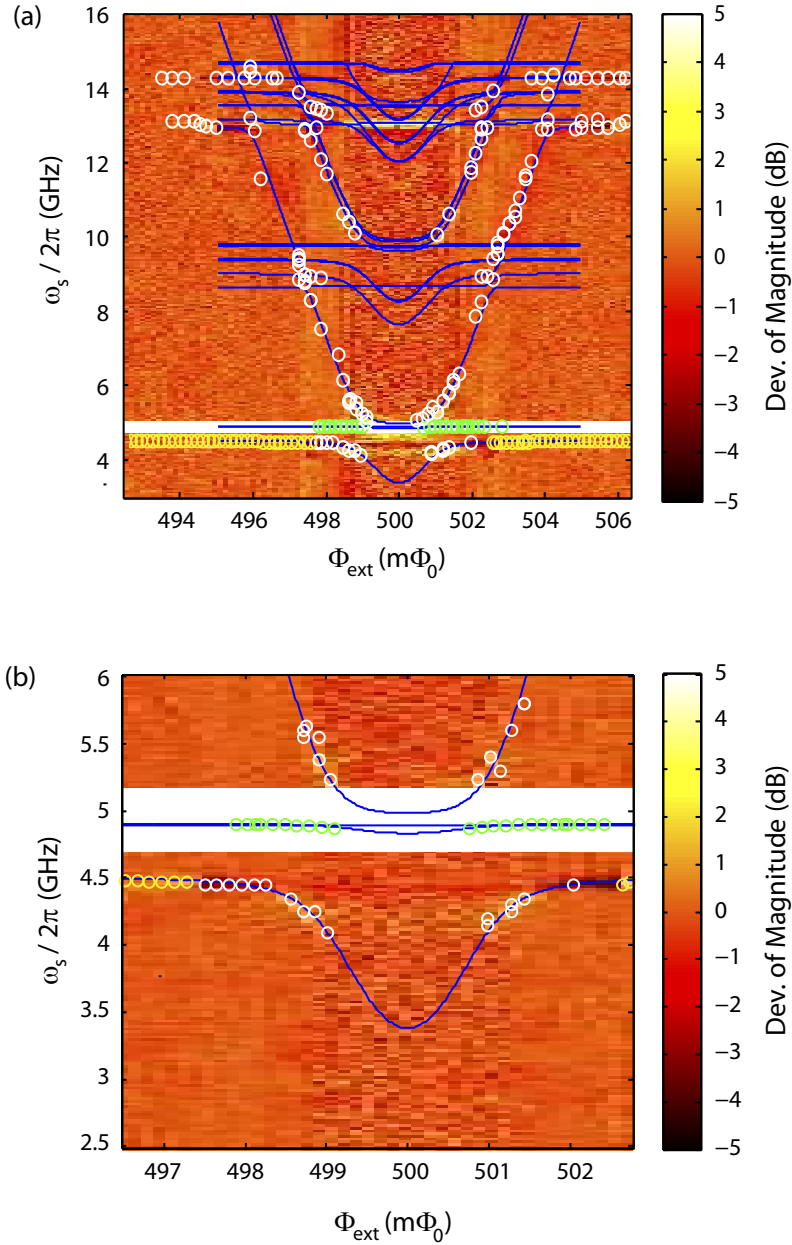
Figure 5.12: Fit (blue lines) of the spectrum of Hamiltonian (5.3) to the data from Fig. 5.7 ( T = 50 mK, P_{\text{rf}} = -20 dBm, \omega_{\text{rf}} = 4.901 GHz, P_{\text{s}} = -5 dBm [Fig. 5.7(a)] and P_{\text{s}} = -17 dBm [Fig. 5.7(b)]) (white circles) and Fig. 5.8 ( T = 50 mK, P_{\text{rf}} = -20 dBm) (yellow circles). Transmission data on the \omega_{+} -mode is indicated by green open circles ( T = 50 mK, P_{\text{rf}} = -20 dBm).
